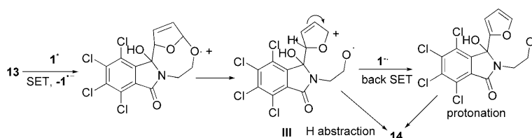
Scheme 2. Proposed mechanism for the formation of 14 .
