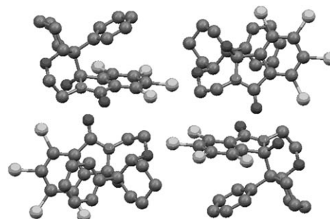
Figure 3. Packing diagram of product 10 .
