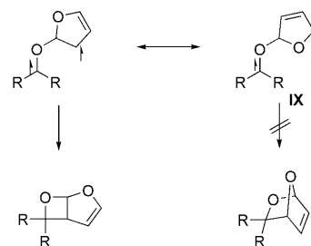
Scheme 6. Biradical intermediates in furan's Paterno–Büchi reaction.
