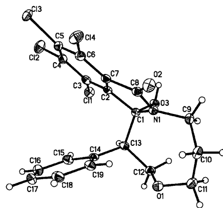
Figure 5. ORTEP drawing of 17 .
