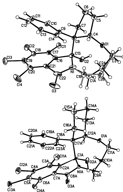
Figure 6. ORTEP drawing of compounds 22 (above) and 24 (below).
