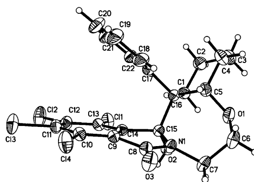
Figure 2. ORTEP drawing of product 10 .
