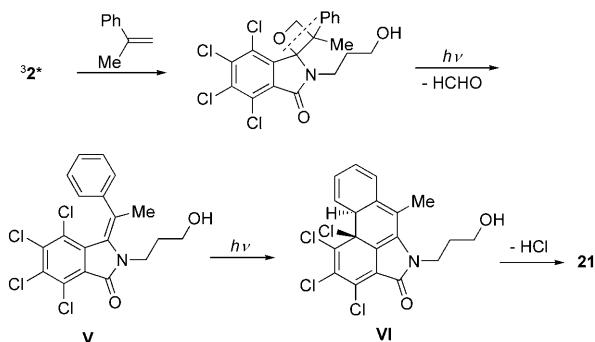
Scheme 4. Proposed mechanism for the formation of 21 .
