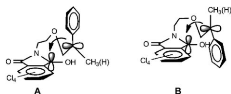
Scheme 7. Left) ISC conformation leading to product 4 (or 7 ). Right) ISC conformation leading to product 5 (or 6 ).
