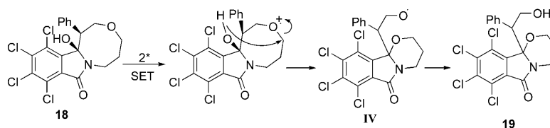
Scheme 3. Proposed mechanism for the formation of 19 .
