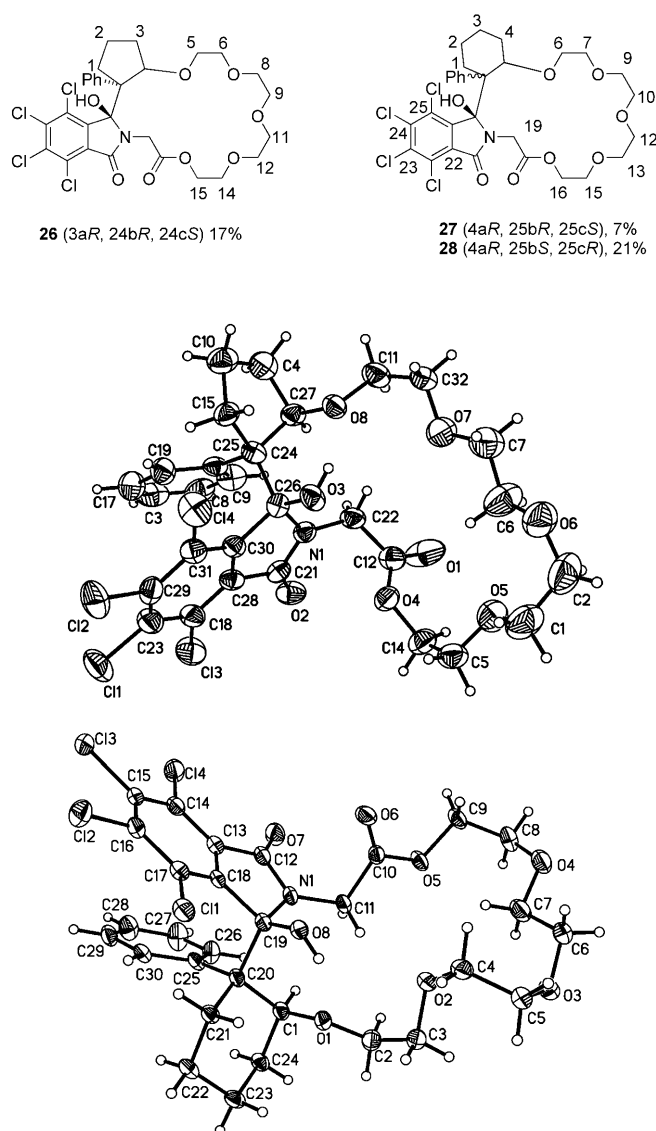
Figure 7. ORTEP drawing of 26 (above) and 27 (below).
