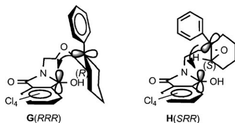
Scheme 9. Left) ISC conformation leading to a (4 aR ,13 bR ,13 cR ) product. Right) ISC conformation for a (4 aS ,13 bR ,13 cR ) product.
