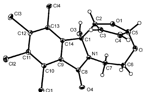
Figure 4. ORTEP drawing of 13 .
