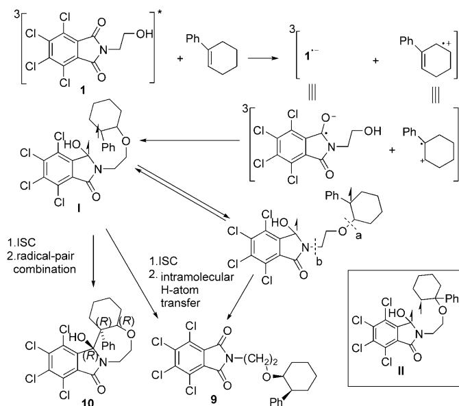
Scheme 1. Proposed photocyclization mechanism.
