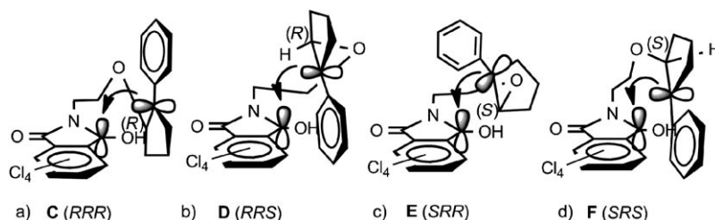
Scheme 8. a) ISC conformation leading to product 8 (3 aR ,12 bR ,12 cR ). b) ISC conformation for a (3 aR ,12 bR ,12 cS ) product. c) ISC conformation for a (3 aS ,12 bR ,12 cR ) product. d) ISC conformation for a (3 aS ,12 bR ,12 cS ) product.
