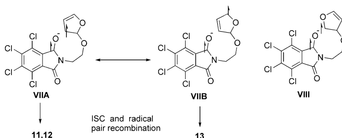
Scheme 5. Formation of 11 , 12 , and 13 from biradical intermediates.
