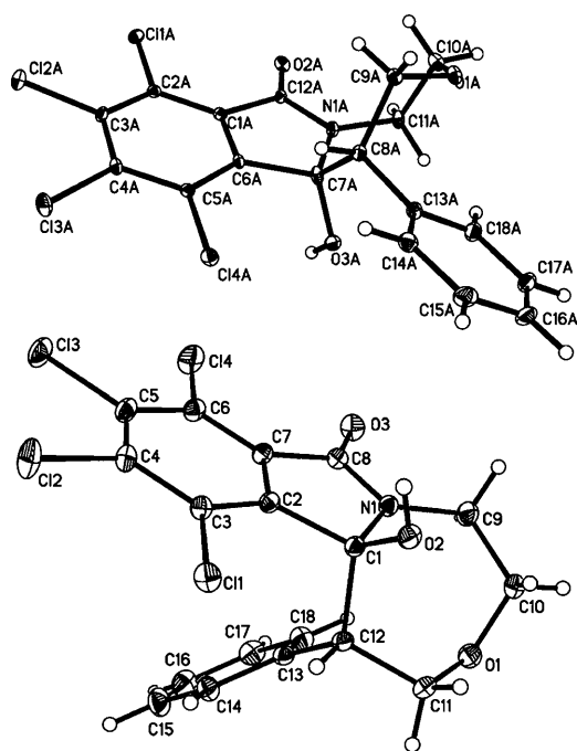
Figure 1. ORTEP drawing of compounds 6 (above) and 7 (below).
